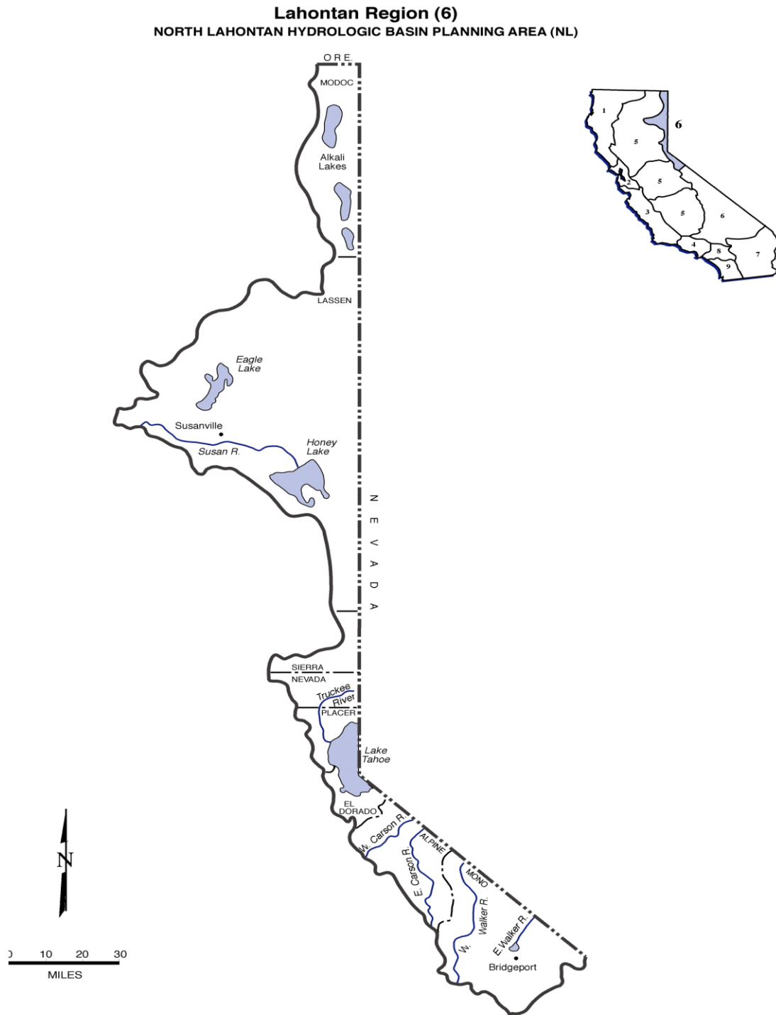
Figure 17. Lahontan Region, North Lahontan Hydrologic Basin.
