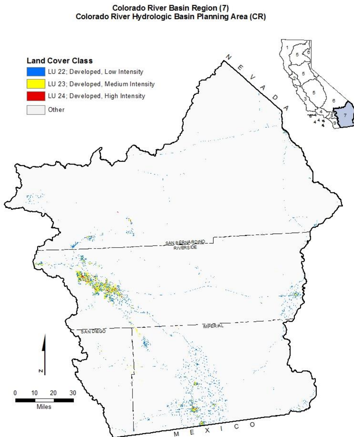
Figure 22. Colorado River Region Developed Land Coverage.
