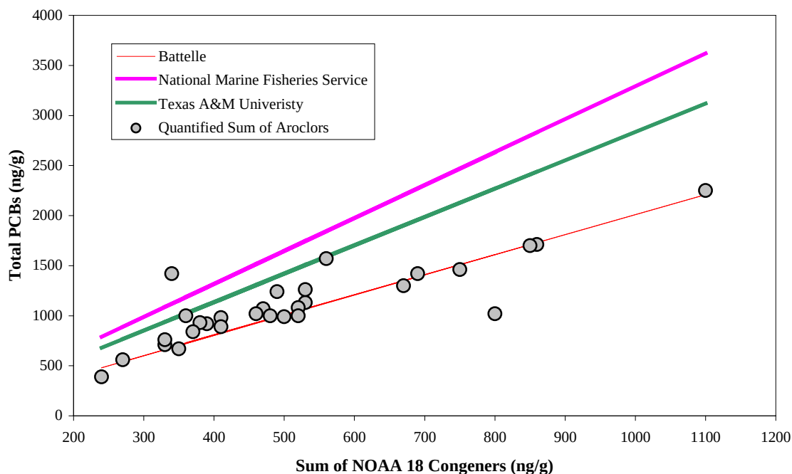
Figure 4-Correlation of PCBs Quantified as Aroclors and Aroclors Calculated from Congener Data (data from SFPUC, 2002).
