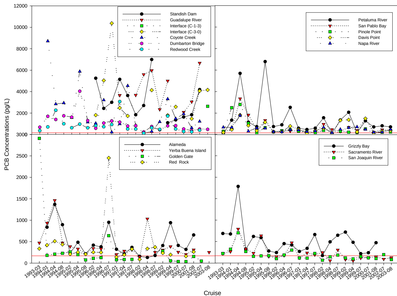
Figure 11-Water Column PCBs Concentrations in San Francisco Bay Fixed Stations (1993-2003)
