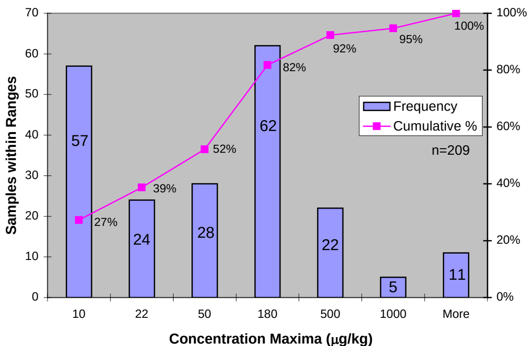
Figure 20-Sediment PCBs Concentrations Distribution in Urban Conveyance Systems (2000-2001)
