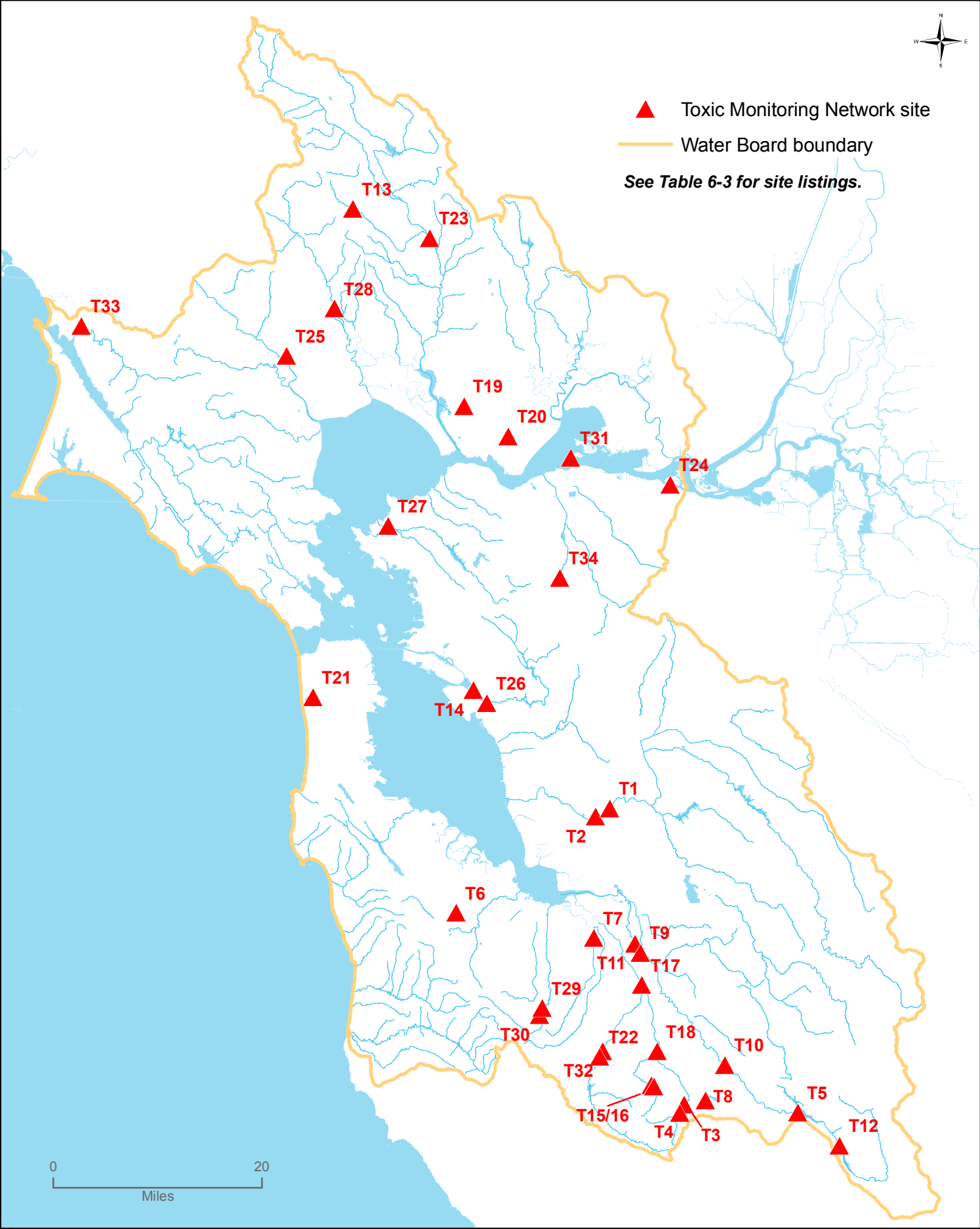
Figure 6-3 Toxic Substances Monitoring Network
